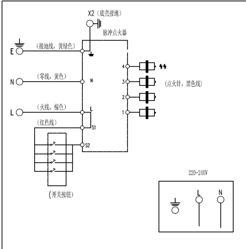
Circuit diagram B for model S46038A, S46038B, S46038C, S46036
