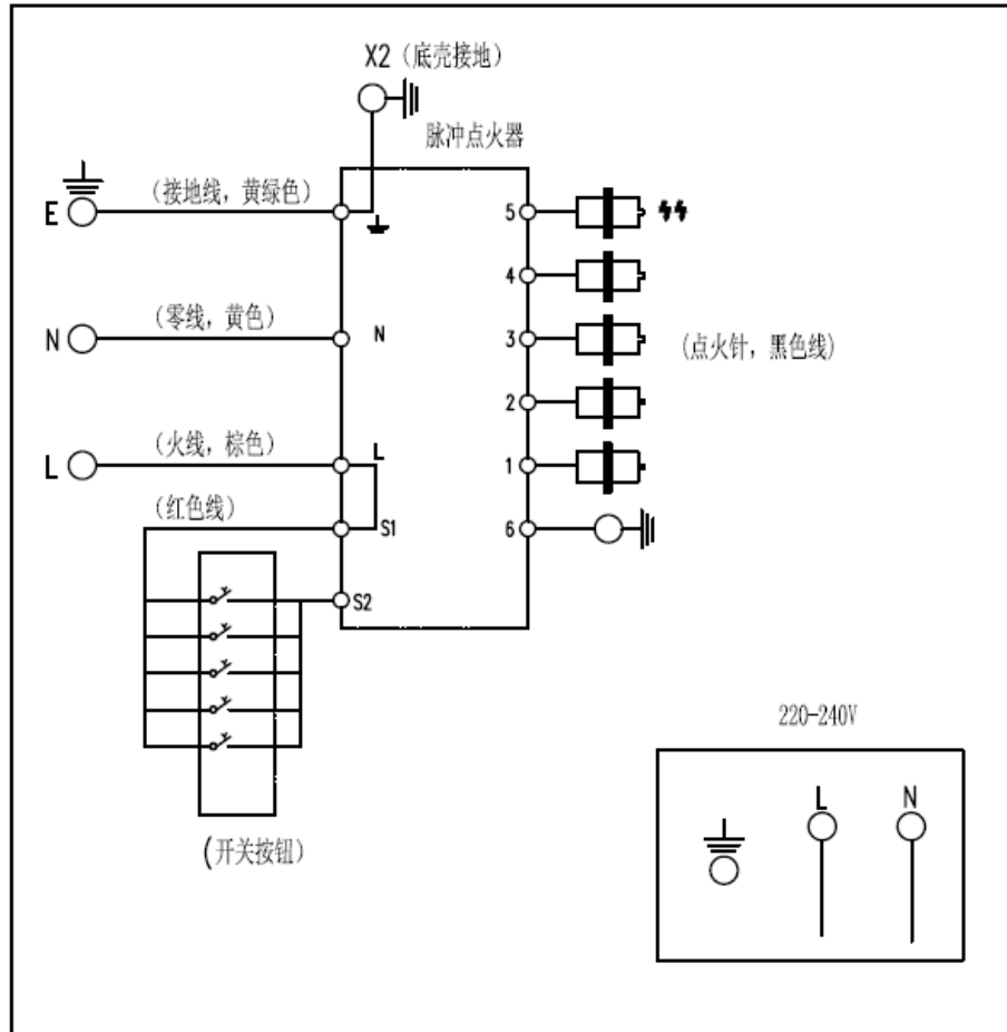
Circuit diagram A for model S58666, S58668A, S58668B, S58668C
