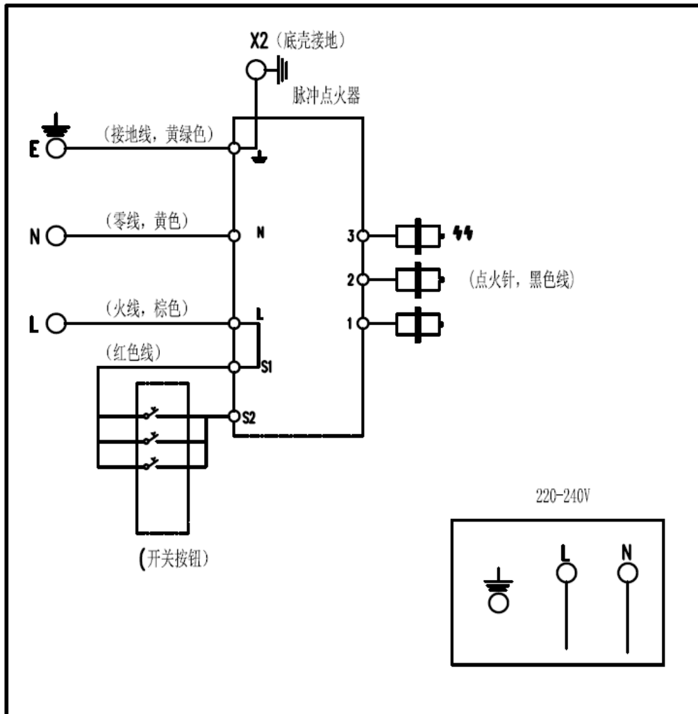
Circuit diagram C for model S38628A, S38628B, S38628C, S38626
